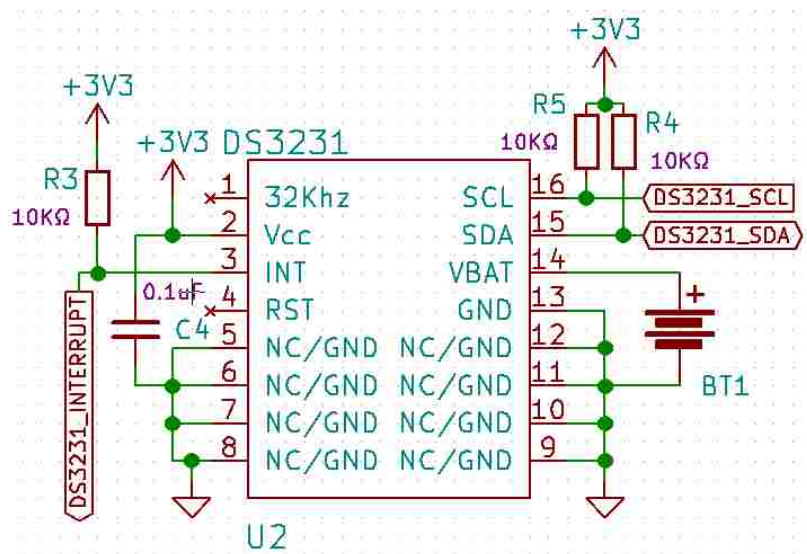
Figure 2.7: Schematic for the DS3231 Real Time Clock. The included coin cell battery allows the device to keep time when the board isn't powered.
